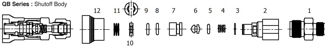
Single-End Shutoff (SESO) No Shutoff Stem Coupled with Standard Shutoff Body
