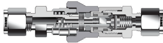
Double-End Shutoff (DESO) Shutoff Stem Coupled with Standard Shutoff Body
