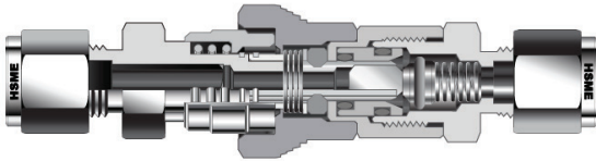
Single-End Shutoff (SESO) No Shutoff Stem Coupled with Standard Shutoff Body
